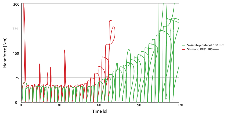
Endurance Test: Handforce
